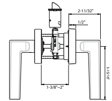
SOHO RC (SH) US26 Round Rosette
