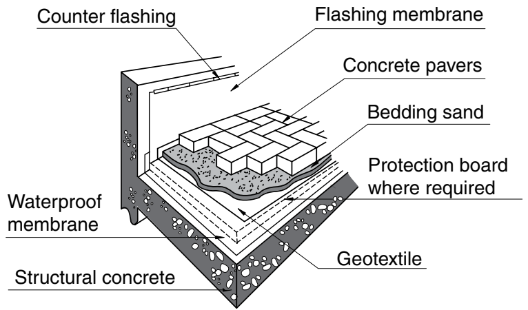
Figure 3. Roof assembly
