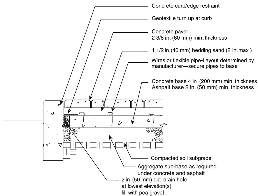
Heated sidewalk/residential driveway on asphalt or concrete base
