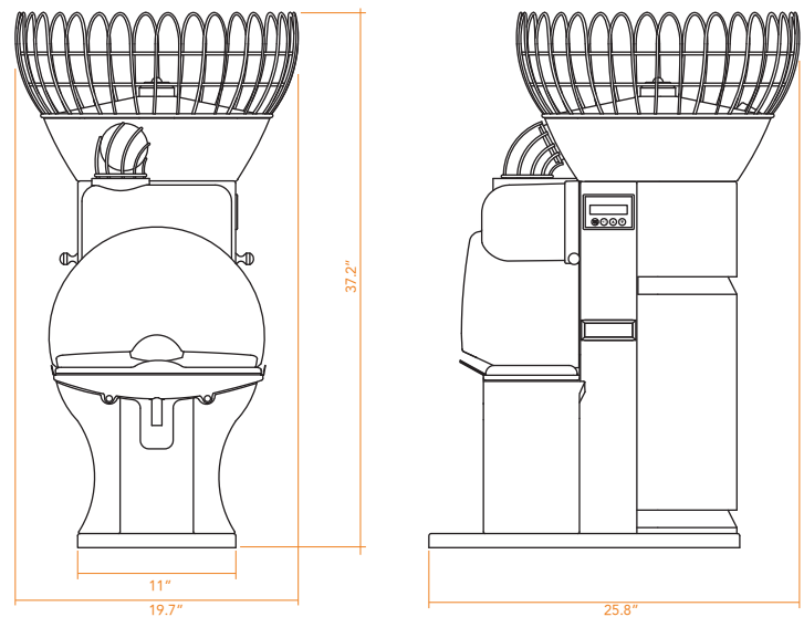
CITROCASA Fantastic F/D – Technical Specifications
