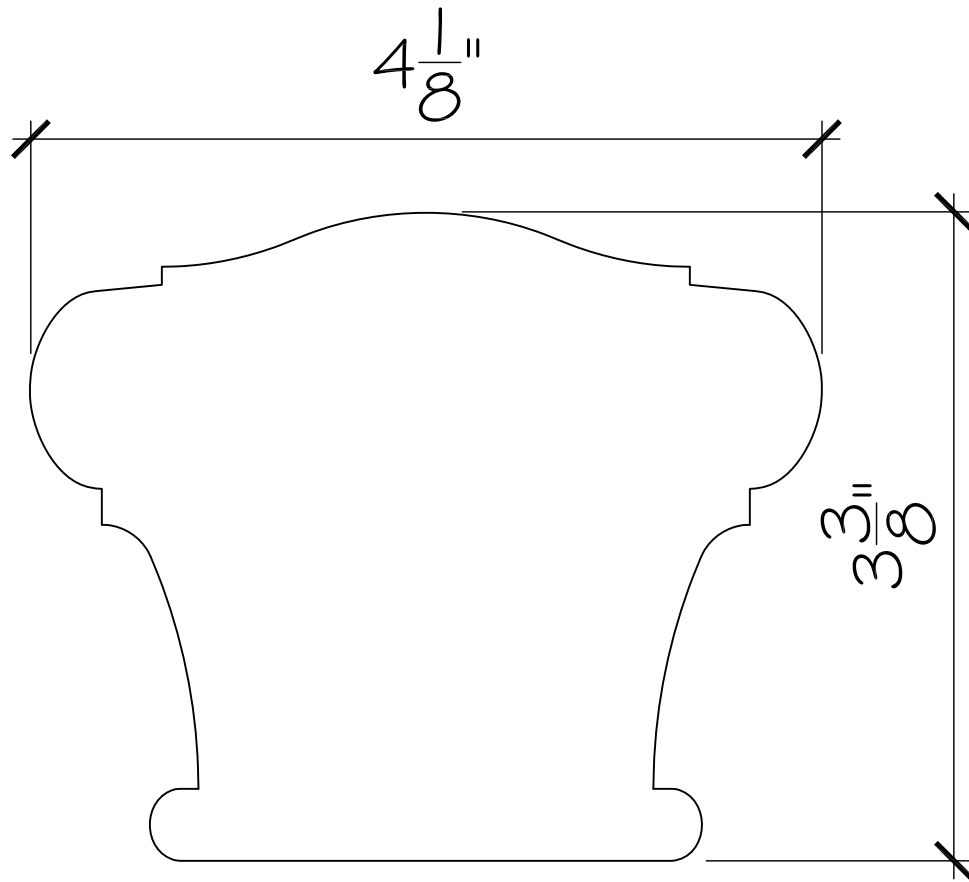
QS 7050 Straight Rail Only
