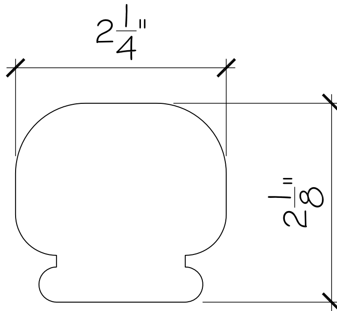
QS 9020 Straight Rail Only
