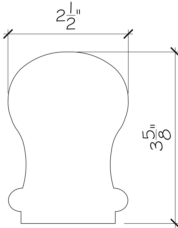
QS 515 Straight Rail Only
