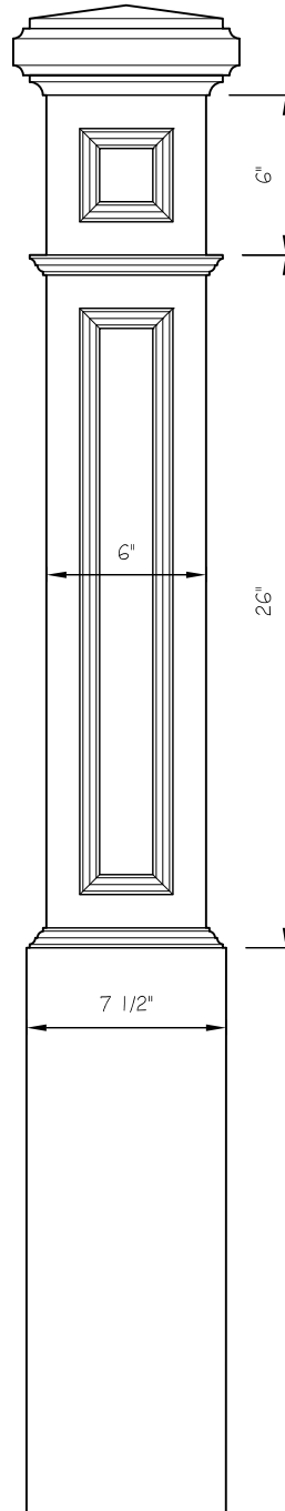
QS - 6" x 6" DOUBLE RECESSED PANEL NEWEL POST WITH #5 CAP
