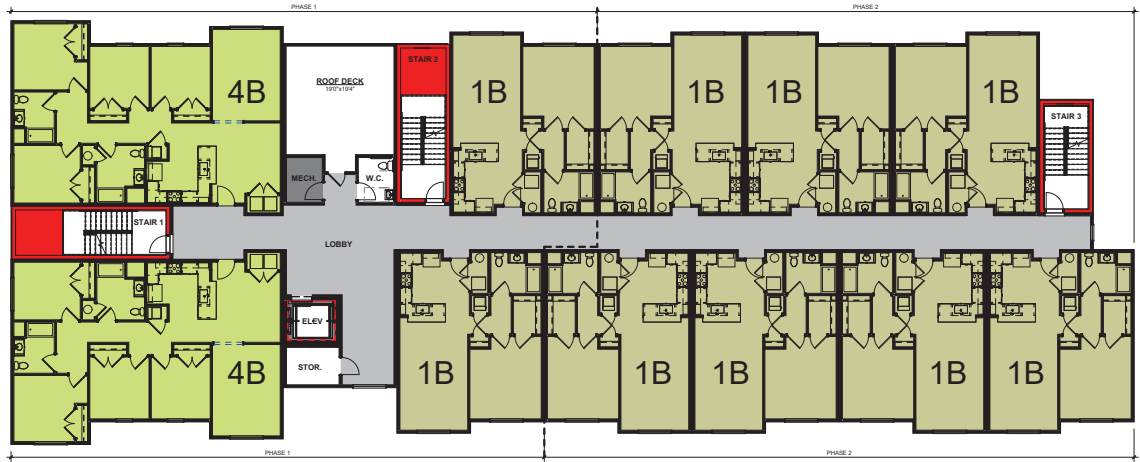
Building 3rd Floor Plan Scale: 1/8" = 1'-0"
