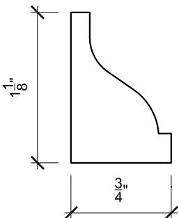
QS Trim # 8 Knives Only
