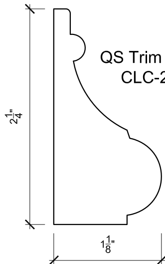
QS Trim # 10 CLC-23
