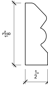
QS Trim # 38 Router Bit
